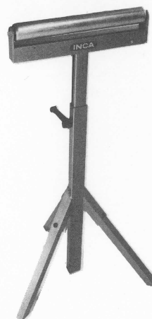
INCA-Rollenbock 348.198.01 Rouleau de support INCA INCA Support Roller
